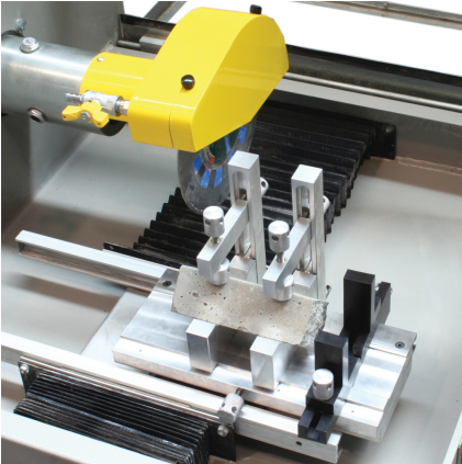
Detail of spindle with clamping mechanism and cutting blade 32-D0536/2
