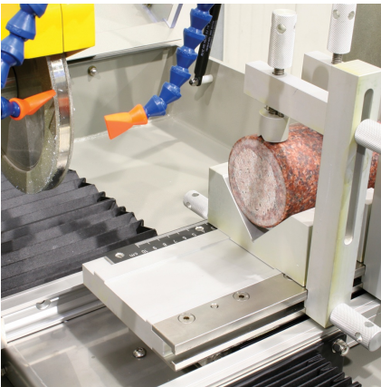
Detail of spindle fit with double-faced diamond cup wheel 32-D0536/3, during surface grinding of cylindrical specimens ends.
