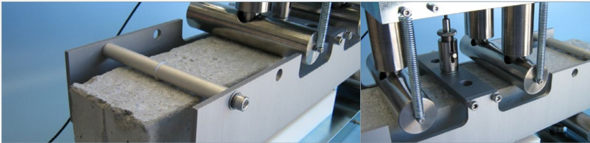
General Purpose Four Point Bending Jig
